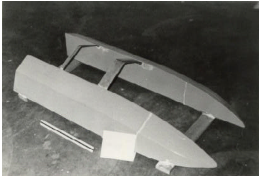
Figure 26: Hysucat Model 6 with Dihedral foils
