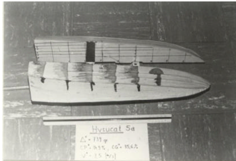
Figure 6. Hysucat model 5a paint tracer test
